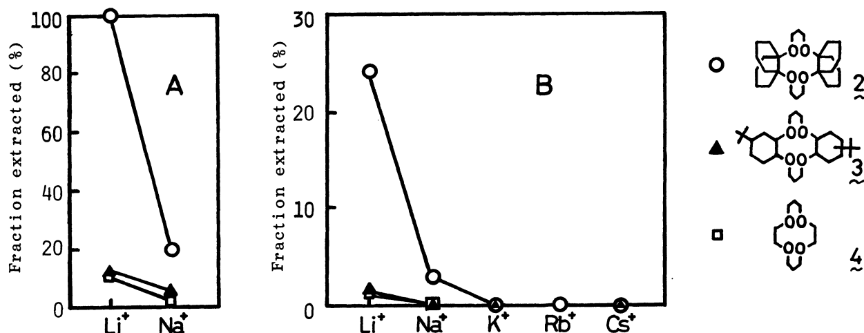
Fig. 1. Extraction of picrates into dichloromethane by crown ethers, 2 , 3 , 6) and 4 . 7) A: [picric acid]= 7.0 \times 10^{-5} M, [crown ether]= 7.0 \times 10^{-4} M, [metal hydroxyde]=0.1 M. B: [picric acid]=[crown ether]= 7.0 \times 10^{-5} M, [metal hydroxide]=0.1 M.
